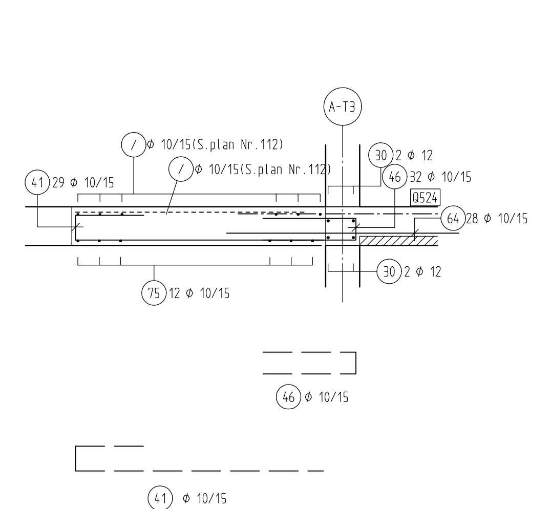
SNITT 12-12, M=1:25
