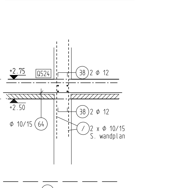
SNITT 8-8, M=1:25
