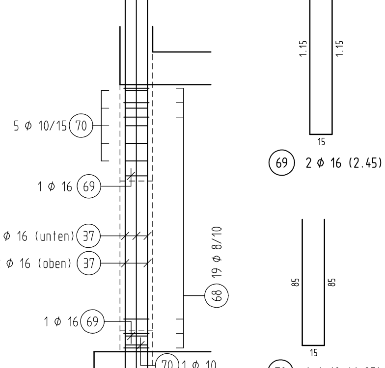
DETAIL A, M=1:25
