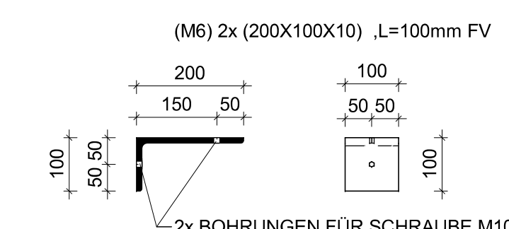
DETAIL "C"
