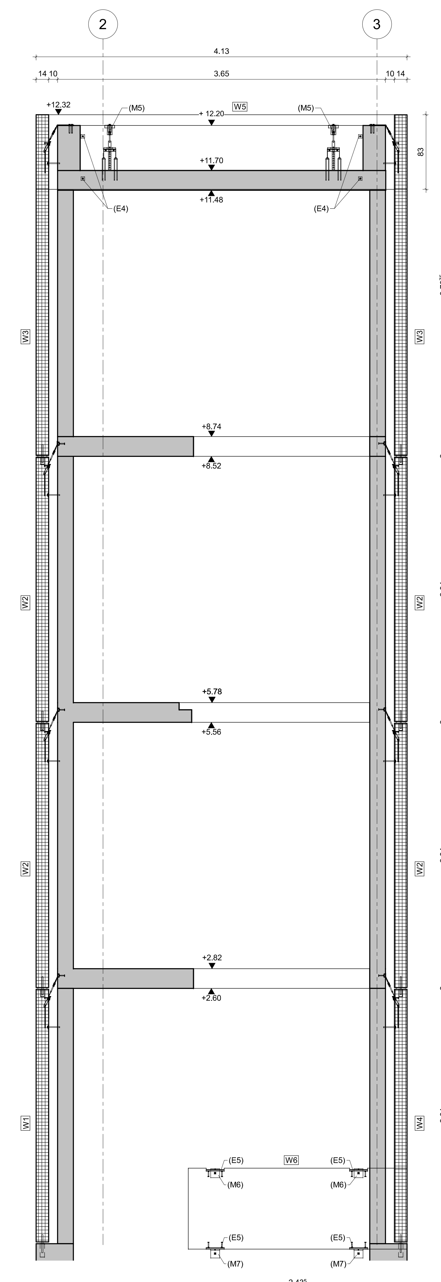
DETAIL "C"
